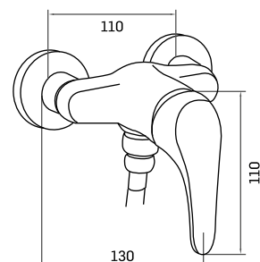
REF. 40027001C. 77 STYLO Monocomando Sanita/Bidé
