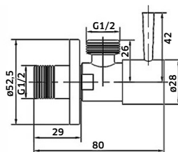
REF. 600010CB. 28 - Branco Kit Shut-Off - 1 Água
