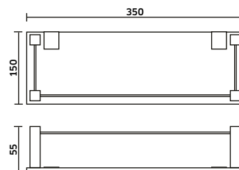
REF. PR035CR. 68 Prateleira 350x150
