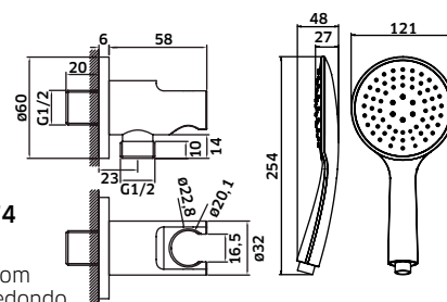
REF. 943023. 59 Cromado REF. 943023PR. 74 Preto
