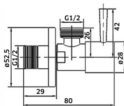
REF. 600010C. 36 - Cromado Kit Shut-Off - 1 Água
