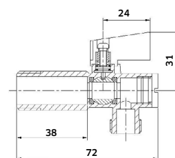
REF. 40013L 1/2*3/8. 3,88 REF. 40014L 1/2*1/2. 3,88 Torneira Esquadria c/ Filtro Longa
